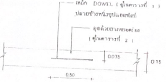
CONTRACTION JOINT
